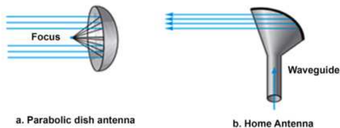
Figure 2.18 Unidirectional antenna
