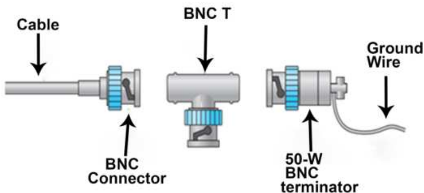
Figure 2.11 BNC connector
