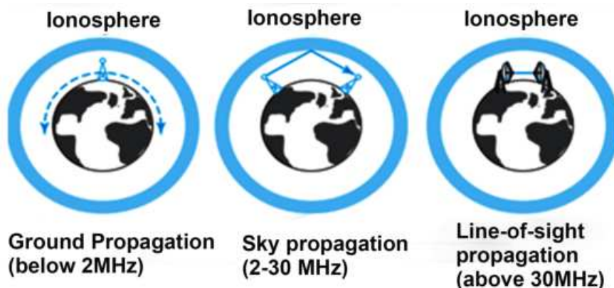
Figure 2.16 Propagation methods
