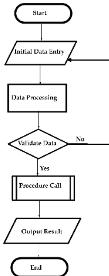
Figure 6.5 Flowchart techniques
