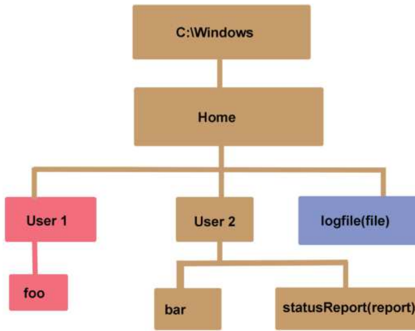
Figure 1.10 Directory structure
