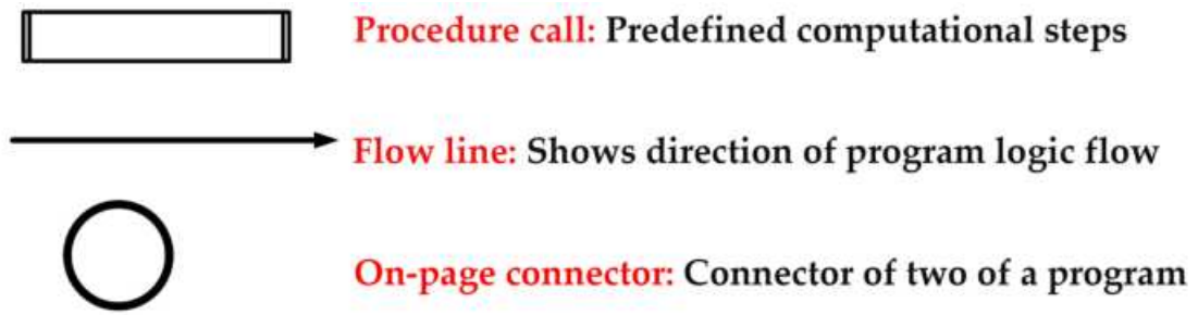
Figure 6.4 Flowchart symbols
