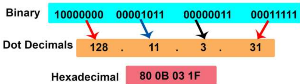
Figure 2.39 Three different notations in IPv4 addressing
