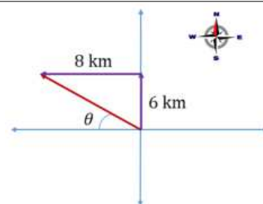
Figure 1.10 displacement of two vectors.
