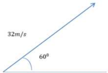
Figure 1.2 vector \vec{v}
