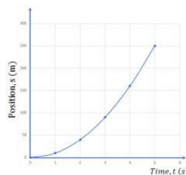
Figure 2.4 Position-time graph.
