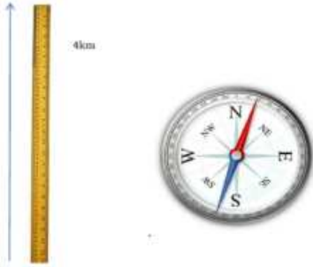
Figure 1.1 Vector \vec{s}
