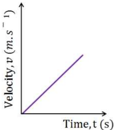
Figure 2.7 Velocity - time graph.
