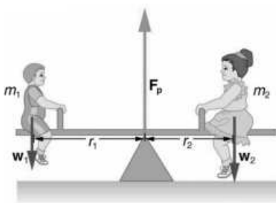
Figure 3.3 The two children in balance.
