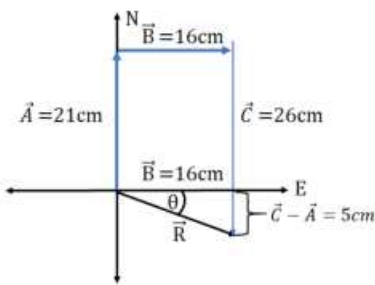
Figure 1.17 The magnitude and direction of the resultant vector.
