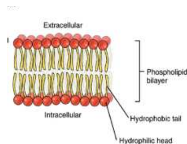
Figure 3.9 Phospholipid bilayer
