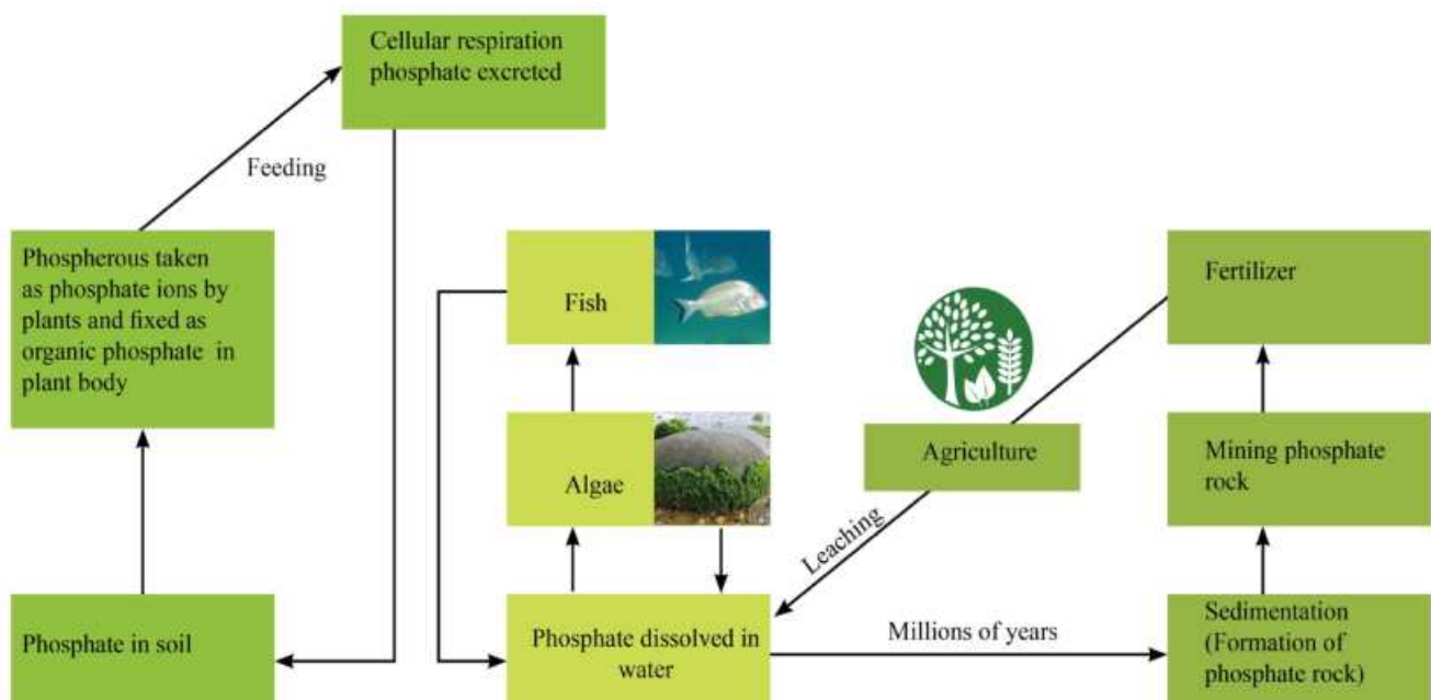
Figure 6.12. Phosphorous cycle
