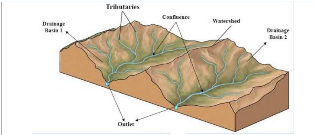
Figure 3.1: Drainage Basin and its Parts
