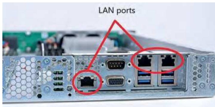
Figure 5.16: LAN ports
