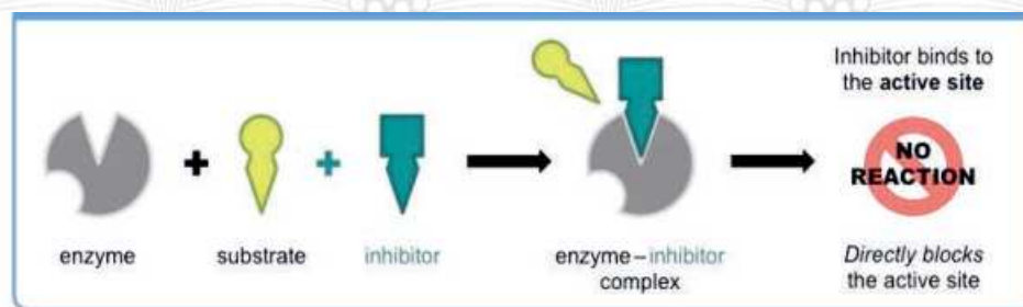
Figure 3.16 Competitive inhibition
