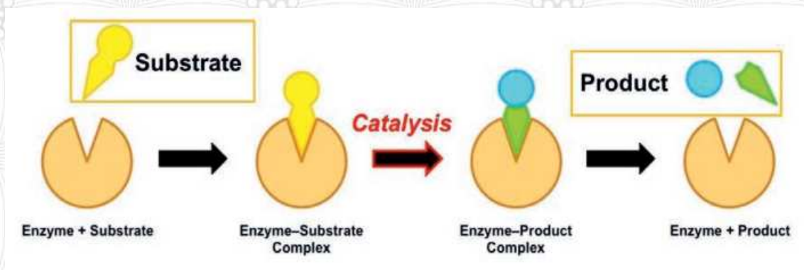
Figure 3.1 Enzymatic reactions
