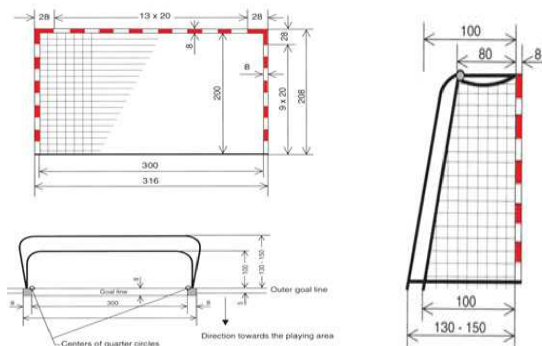
Figure 7.1 a) Handball Goal front view b) lateral view (Dimensions indicated in centimetre)
