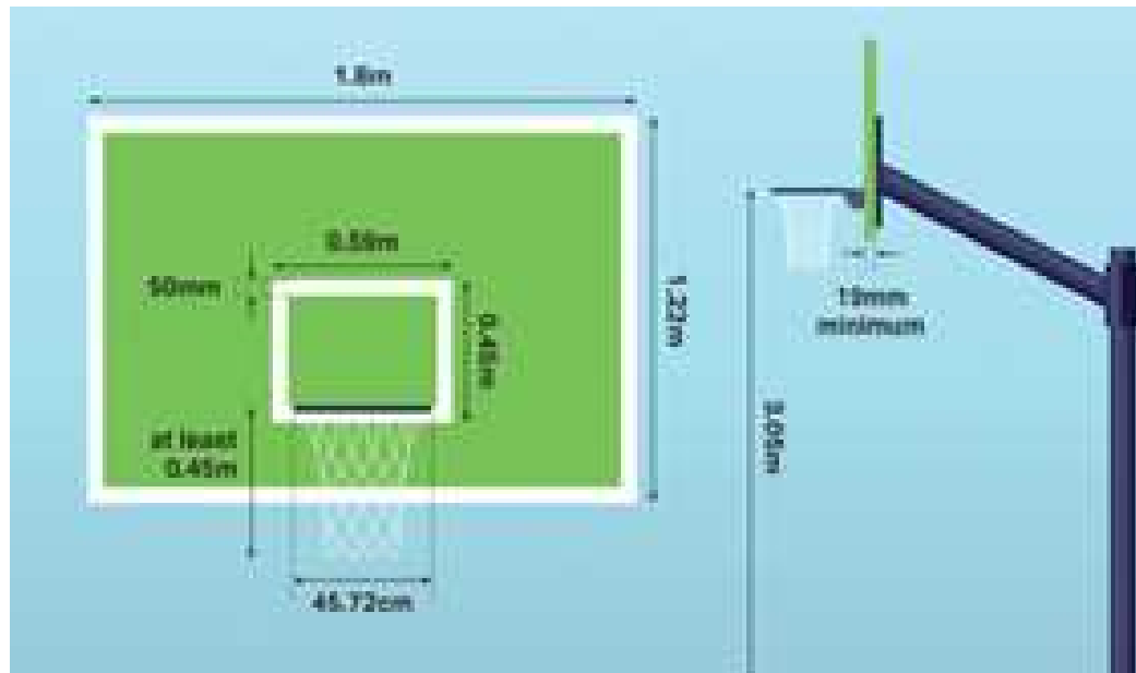
Figure 6.4. Basketball Backboard
