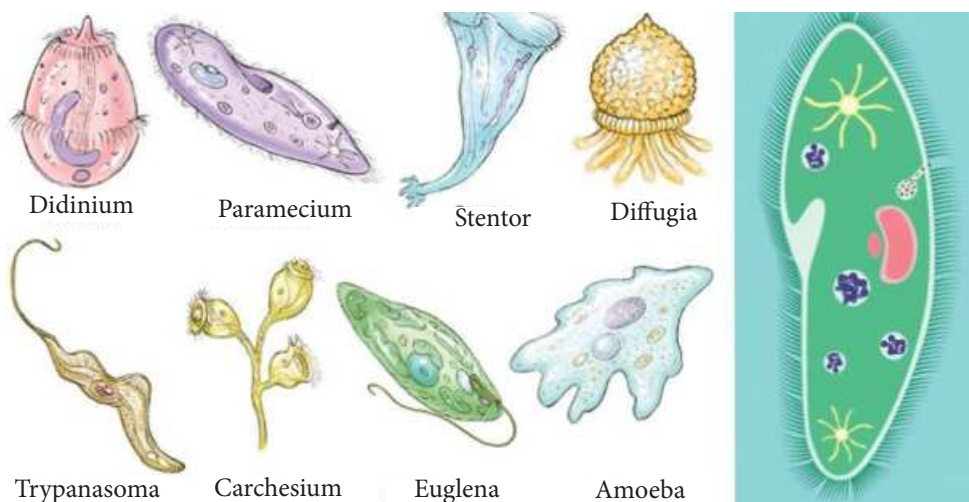
figure 5.11 Protista
