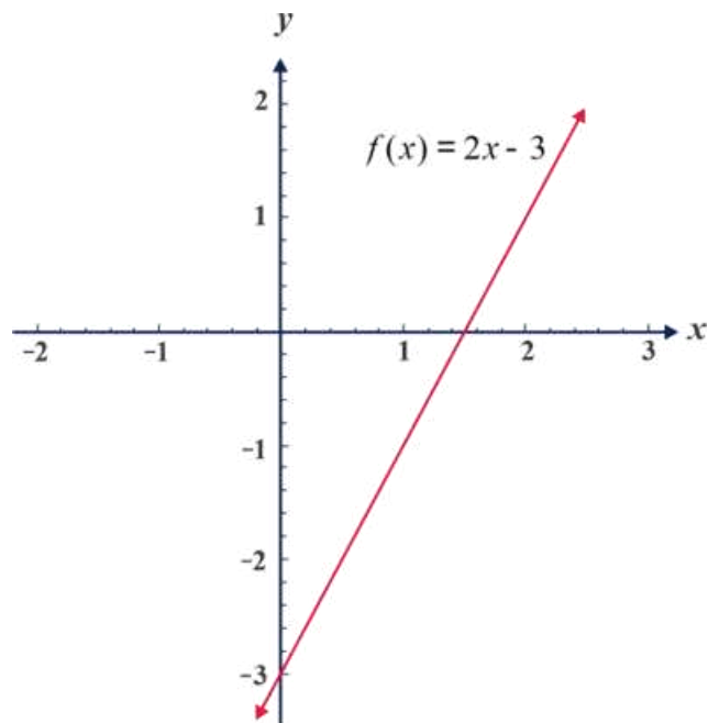
Figure 1.26 The graph of f(x) = 2x - 3
