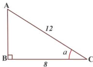
Figure 4.44 Right-angled Triangle
