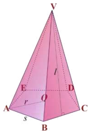
a. Regular pentagonal Pyramid
