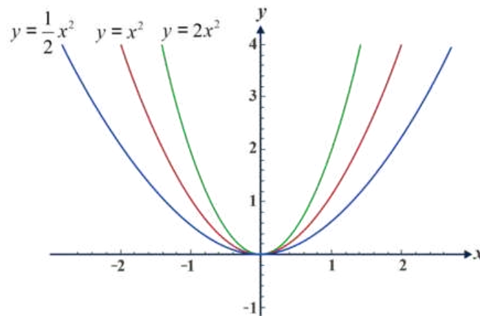
Figure 1.29 the graph of y = ax^2 , a = \frac{1}{2}, 1, 2
