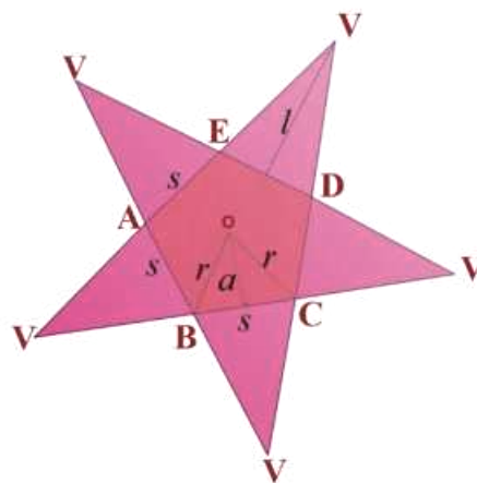
b. Net of Figure a
