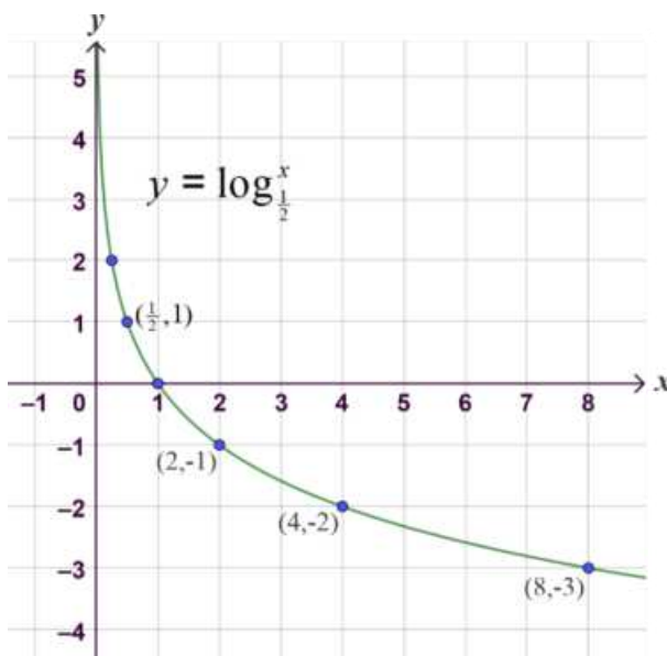
Figure 3.9: Graph of f(x) = \log_{\frac{1}{2}} x
