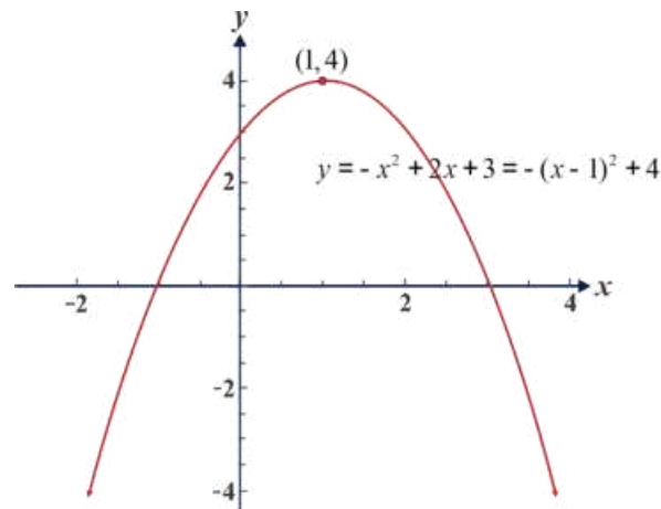
Figure 1.35 The graph of y = -x^2 + 2x + 3
