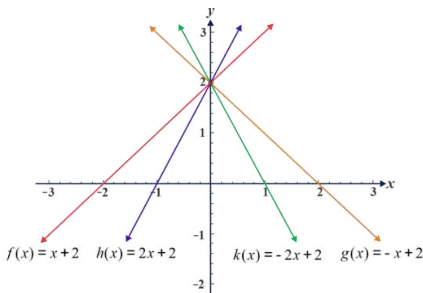
Figure 1.25 The graph of four functions f , g , h , k intersecting at a point (0, 2) .
