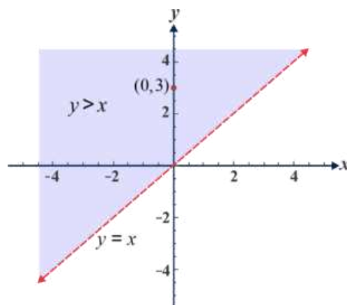
Figure 1.7 The graph of the relation y > x
