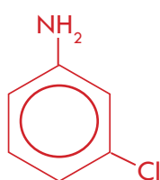
3-chloroaniline (m-chloroaniline)
