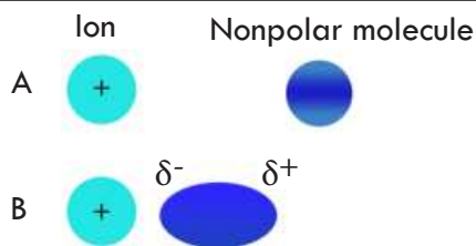
Figure 2.6 Ion–induced dipole interactions. (A) when the ion and the nonpolar molecules are far apart, (B) when the ion and the nonpolar molecule get closer—the nonpolar molecule gets polarized.
