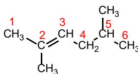
2,5-dimethyl-2-hexene
