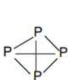
The white phosphorus molecule
