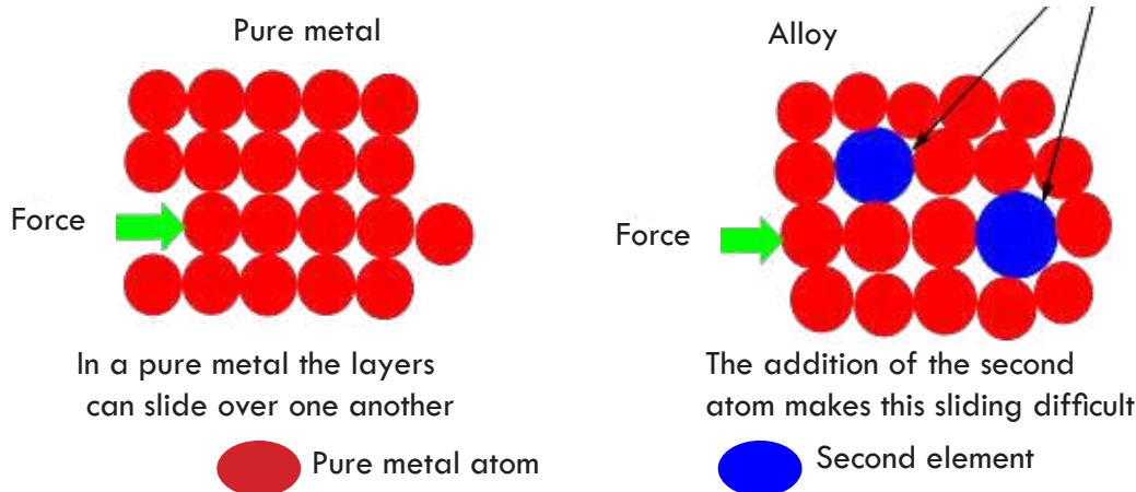
Figure 5.3 Arrangement of metal atoms in pure metal and alloy.
