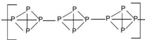
The arrangement of atoms in red phosphorus
