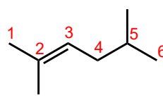
2,5-dimethyl-2-hexene
