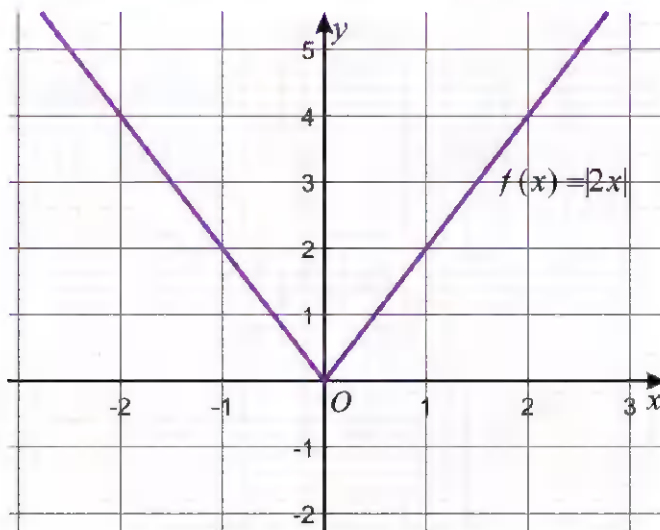
Figure 1.45: Graph of f(x) = |2x|
