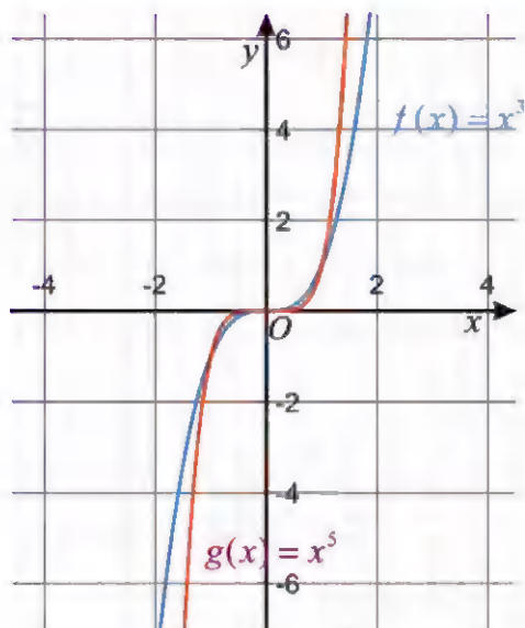
Figure 1.22: Graphs of f(x) = x^3 and g(x) = x^5
