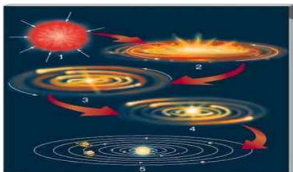
Figure 6.16 The process of the Formation of Solar
