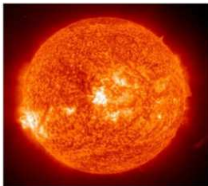
Fig 6.2 The Sun
