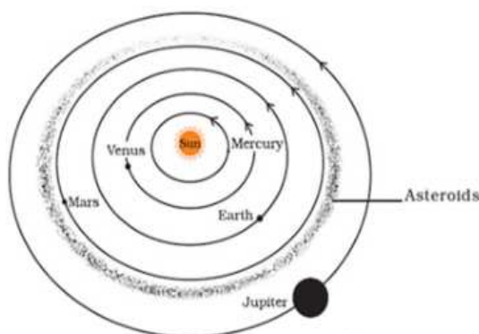
Figure 6.12 Asteroids
