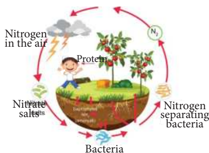
Figure 5.14 Nitrogen Cycle
