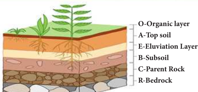
Figure 5.20 soil horizons
