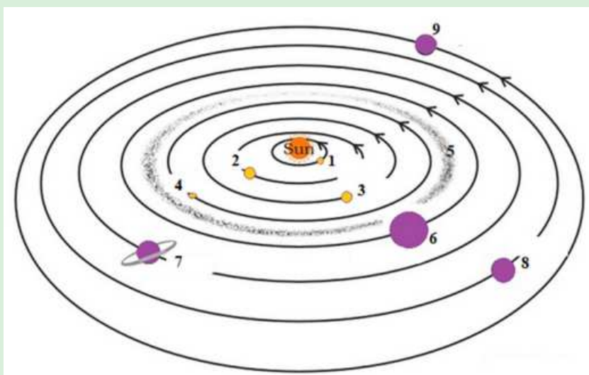
Figure 6.15 Solar system
