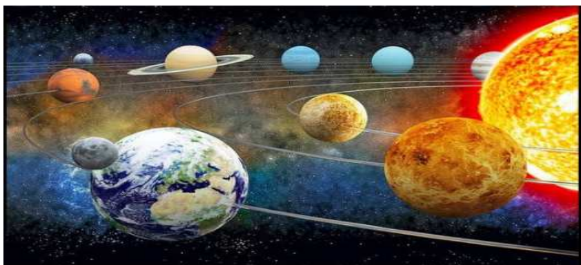
Figure 6.17 Formation of Planets
