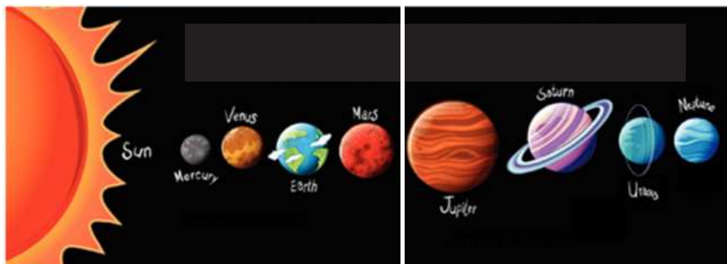
Figure 6.11 (a) Inner planets
