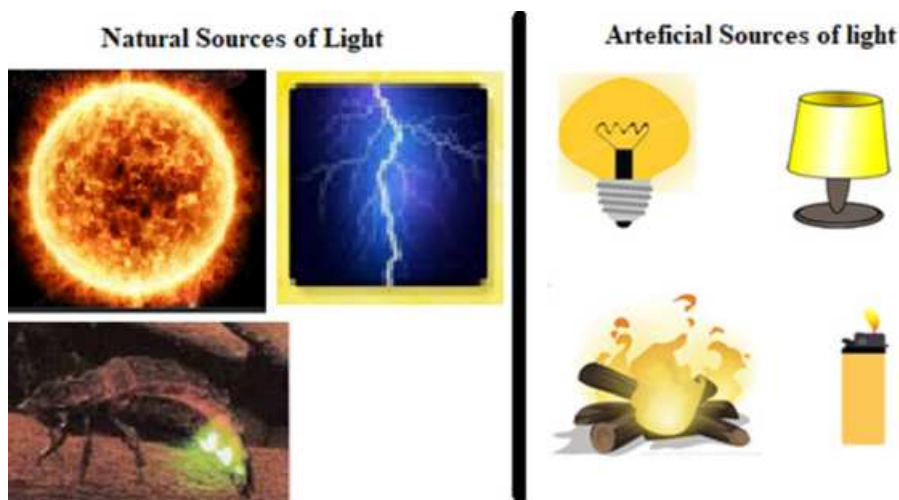
Figure 7.1 Sources of light
