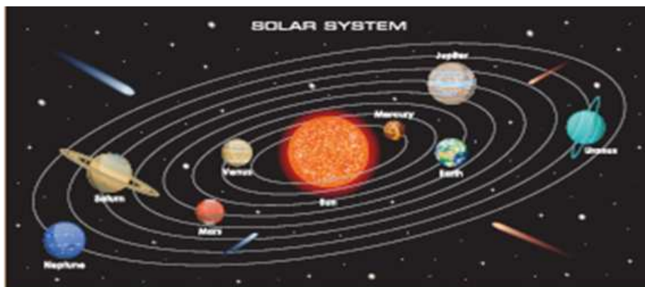
Fig. 6.1 The solar system
