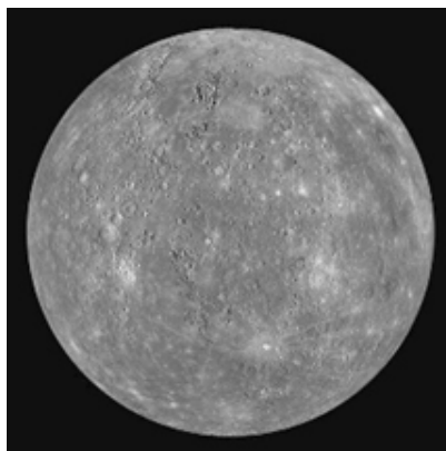
Figure 6.3 mercury
