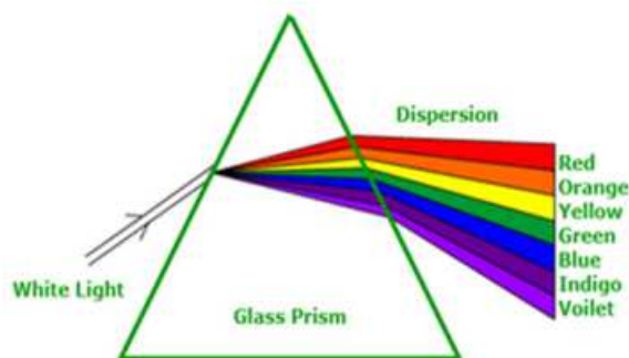
Figure 7.6 Dispersion by a prism
