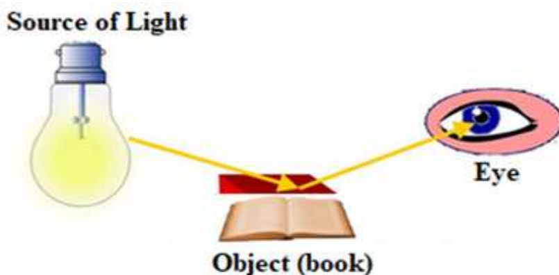
Figure 7.3 Seeing non-luminous objects
