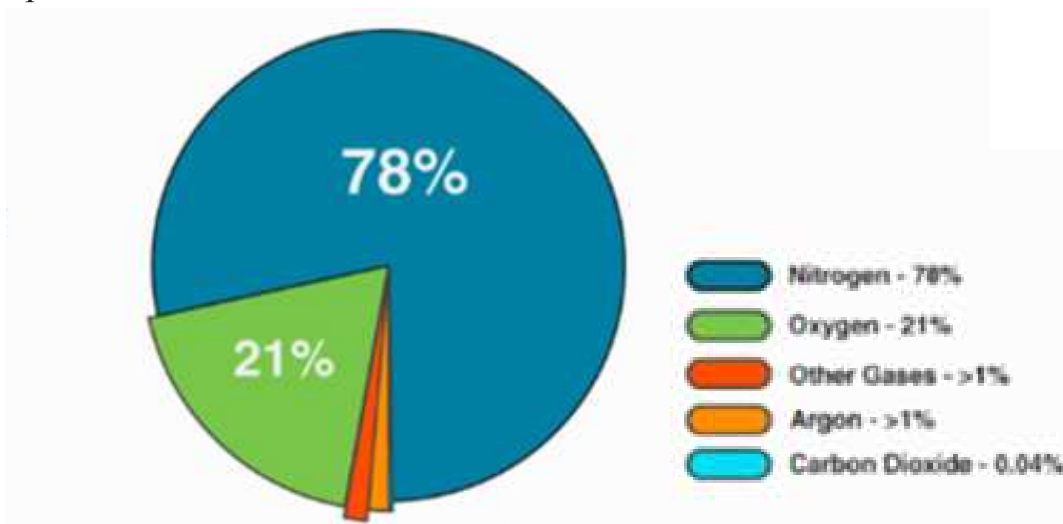
Figure 5.27 air compositions
