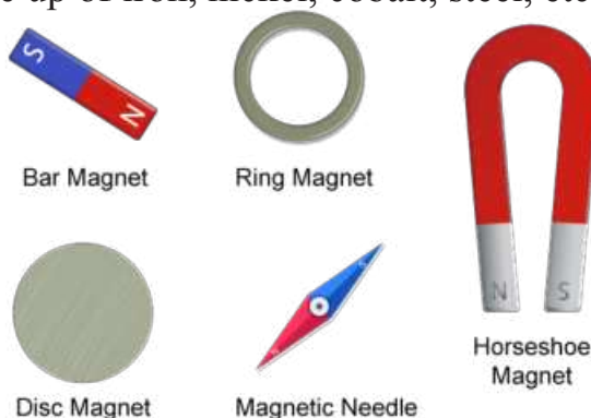
Figure 7.16 Artificial magnet
