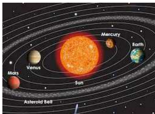
Figure 1.2 Asteroids belt
