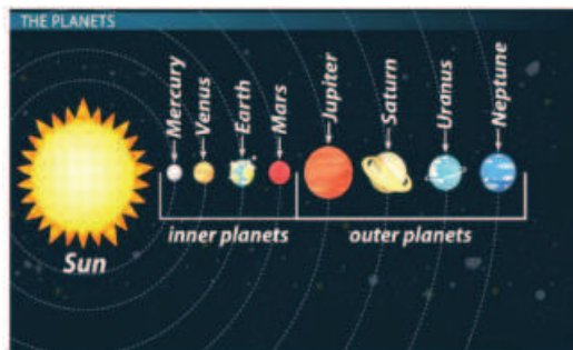
Figure 1.1 The Planets
