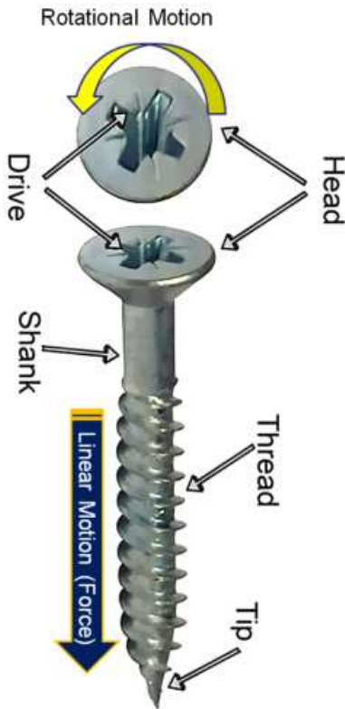
Figure 5.18 The screw.
