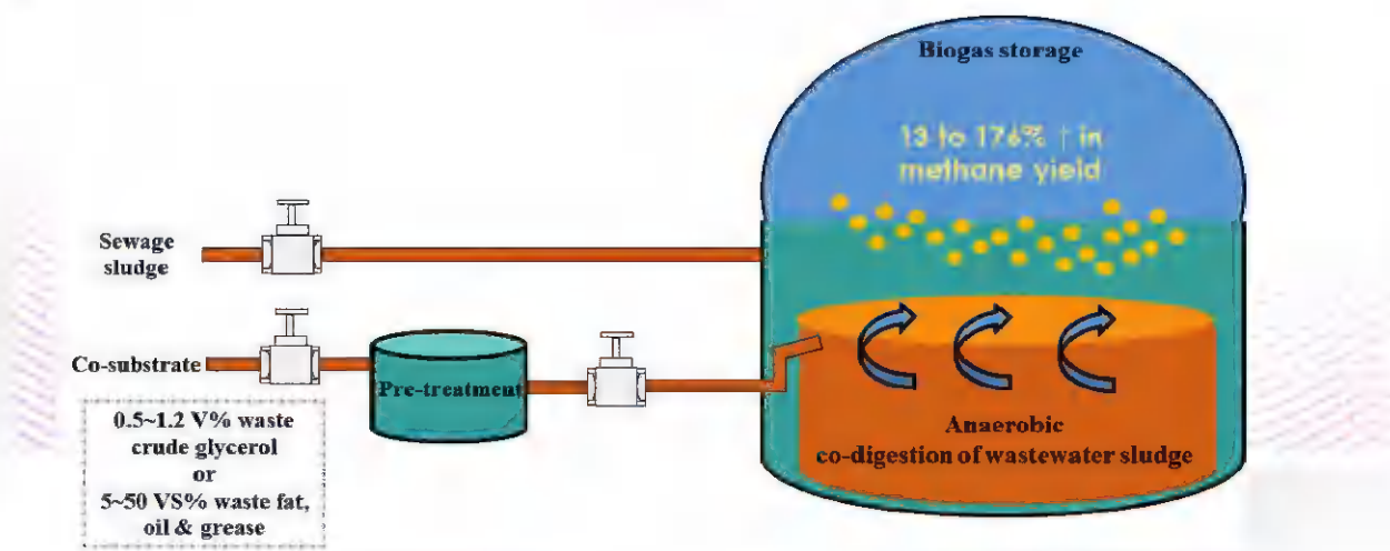
Figure 2.33. Anaerobic co digestion of waste water
