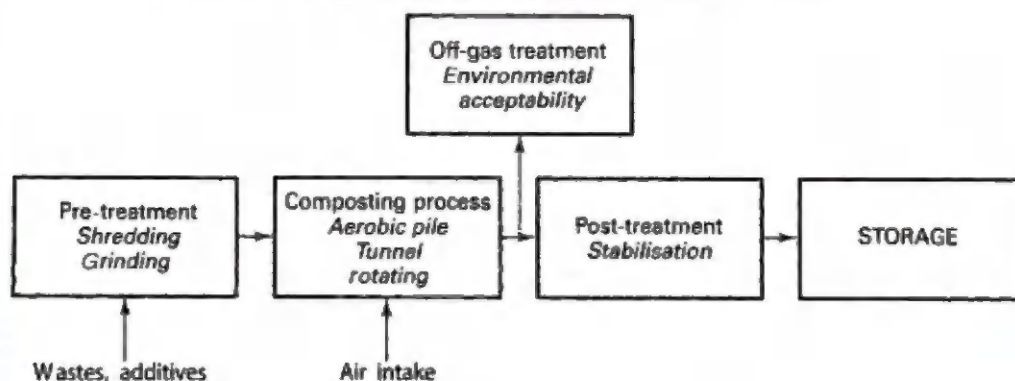
Figure 1.13. flow chart composting plants processes
