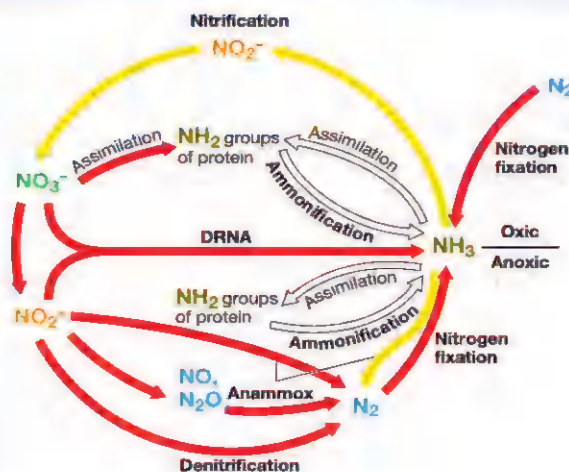
Figure 2.38. The nitrogen cycle
