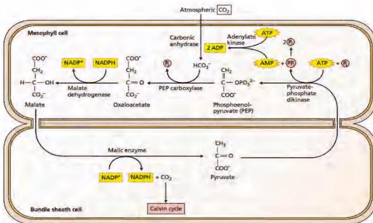
Figure 3.8. The \text{C}_4 photosynthetic pathway
