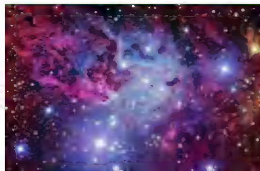
Figure 4.5 Clouds of inter-stellar gas have been shown to contain organic molecules
