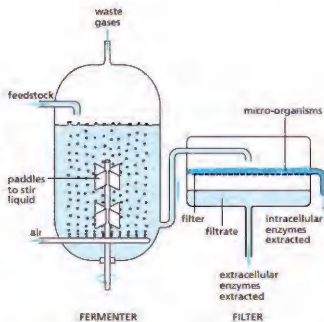
Figure 1.14. Principles of enzyme production from micro-organisms
