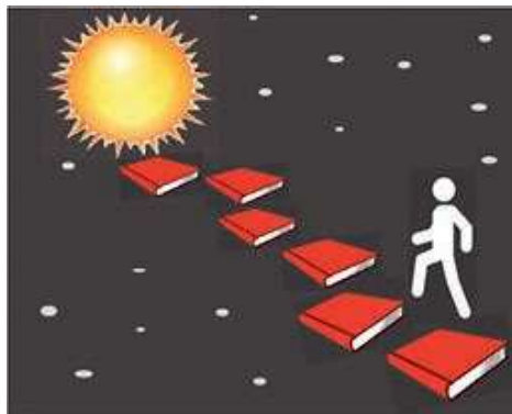
Figure 1.4: Wisdom
