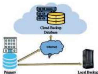
Figure 5.9 Data backup
