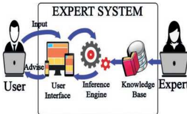
Figure 2.5 Expert system
