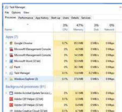
Figure 5.5 Task Manager
