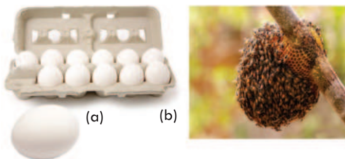
Figure 2.6 (a) A dozen eggs is exactly 12 eggs. (b) A specific swarm of honeybees contains an exact number of live bees (but it would be difficult to count them, and any two swarms would be unlikely to contain the same exact number of bees).
