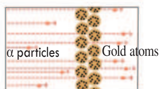
(b) What Rutherford expected if Thomson's model were correct
