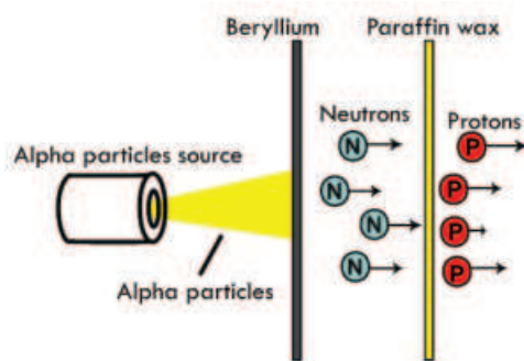
Figure 3.20 James Chadwick's beryllium bombardment experiment.
