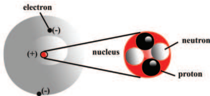
Figure 3.24 The sub atomic particles.
