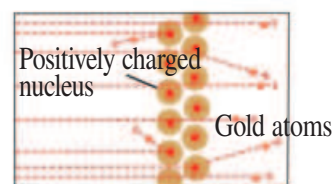
(b) What Rutherford actually observed
