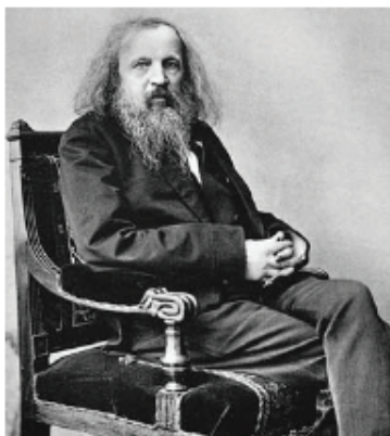
Figure 4.3 Dmitri Ivanovich Mendeleev (1834–1907) Mendeleev constructed a periodic table as part of his effort to systematize chemistry. He received many international honors for his work, but his reception in czarist Russia was mixed. He had pushed for political reforms and made many enemies as a result.
