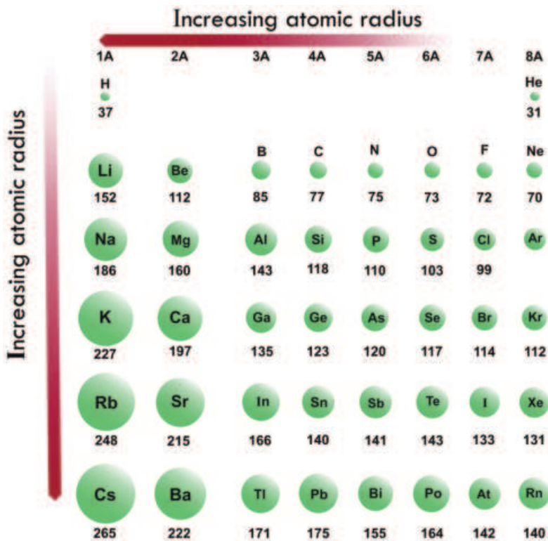
Figure 4.8 Atomic radii (in picometers) of representative elements according to their positions in the periodic table. Note that there is no general agreement on the size of atomic radii. We focus only on the trends in atomic radii, not on their precise values.
