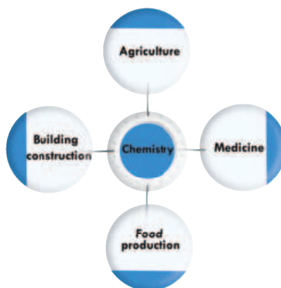
Figure 1.6 The role of chemistry in different sectors.
