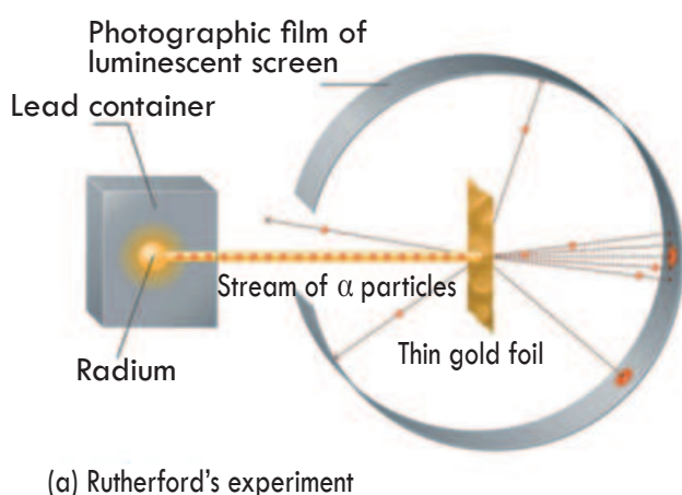
Figure 3.17 A Summary of Rutherford's Experiments.
