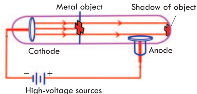
Figure 3.10 Cathode rays creating a shadow of small object on the cathode ray tube screen.
