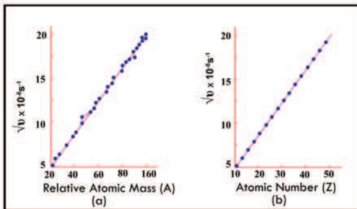
Figure 4.4 Plots obtained in Moseley's experiments.
